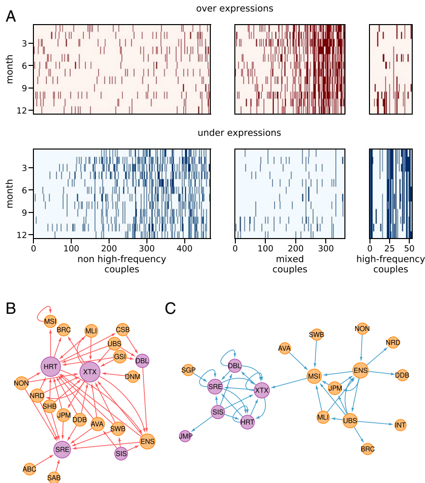
Fig. 2. (A) Time persistence of overexpression or underexpression of each aggressor → counterpart couple observed in the AC statistically validated networks of SKF in the 12 mo of 2018 (vertical scale of the panels). The statistical validations are grouped in three sets. Left sets include couples of market members that are not HFTs, Center sets include couples of market members composed of one HFT interacting with a non-HFT, and Right sets include couples of two HFTs. For Top panels, the presence of a vertical segment indicates overexpression of the number of transactions of the market member couple (labeled by a numerical index) whereas in Bottom panels underexpressions are highlighted. B shows the overexpressed (red arcs) aggressor → counterpart couples detected in 9 or more months of 2018. C shows the underexpressed (blue arcs) aggressor → counterpart pairs detected in 9 or more months of 2018. In B and C , we label nodes with the tick symbol of the market member and we use a purple color when the market member is described as a HFT. The market members that are not explicitly described as HFTs are shown as orange nodes. We use trading ID abbreviations to market members' names, which are the same as used by Nasdaq Nordic (see http://www.nasdaqomxnordic.com/membership-list ).
